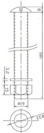
SETTING B/N ( \phi 19 \times 180 )
