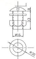
JOINTING B/N ( \phi 16 \times 33 )
